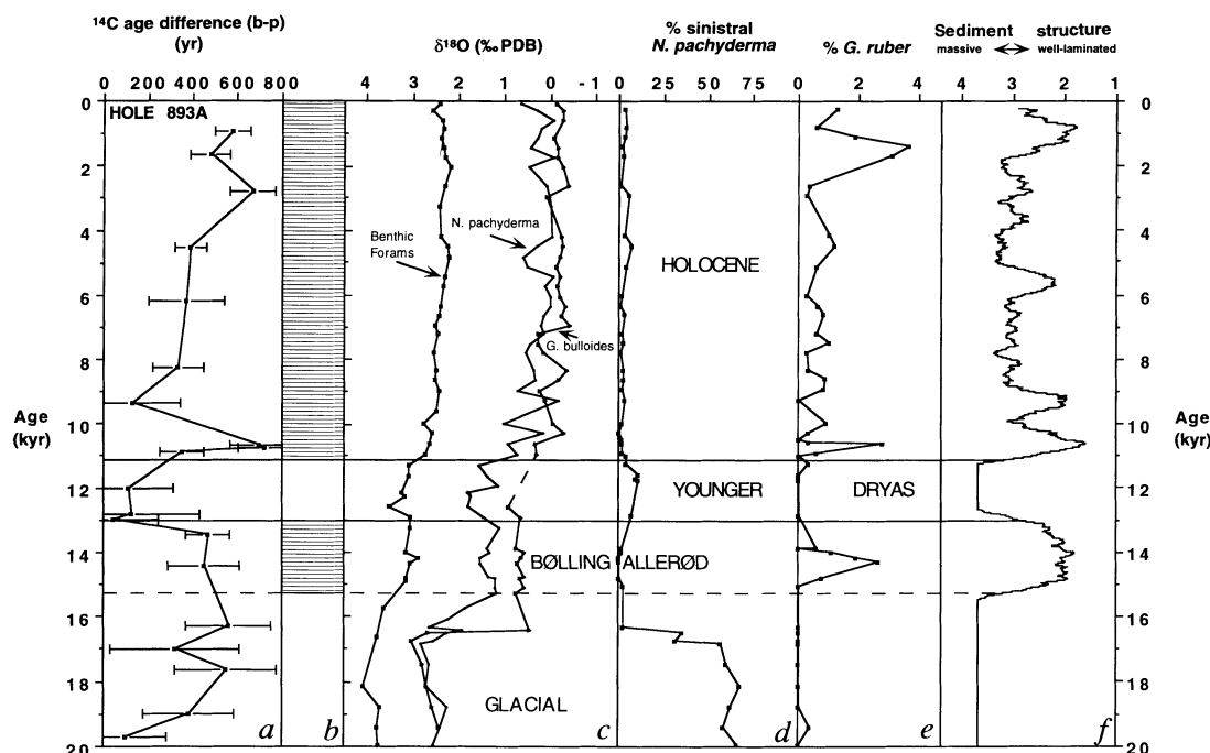
FIG. 1. Relations between inferred age of basinal waters (a), sediment structures (b, f) and palaeoclimate proxies (c, d, e) for the past 20 kyr (upper 32 m of Ocean Drilling Program Hole 893A, Santa Barbara basin, southern California). a, Benthic–planktonic (b–p) age differences ( ^{14}\text{C} ) are considered to represent changes in age of basinal bottom waters 12 . Reservoir-age correction used throughout is 825 yr (ref. 12); insufficient information exists to adjust for probable changes in reservoir ages with time. Chronology after refs 12 and 16. b, Presence (shaded) or absence (unshaded) of sediment laminations. f, Visual description of sediment structures at one-cm resolution for the entire sequence 26 , grading from well-laminated to massive (1, well-laminated; 2, indistinctly laminated; 3, trace laminations; 4, massive or non-laminated). The curve in f was smoothed using a 99-cm running average to reduce variability and exhibit more clearly the major events addressed here. Smoothing has little effect on age of sediment facies transitions. These changes have been correlated to changes in degree of oxygenation and sediment
